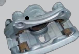
BA/BF FALCON Front/Rear Calipers, including revised pistons and pins to prevent retraction and noise issues.
